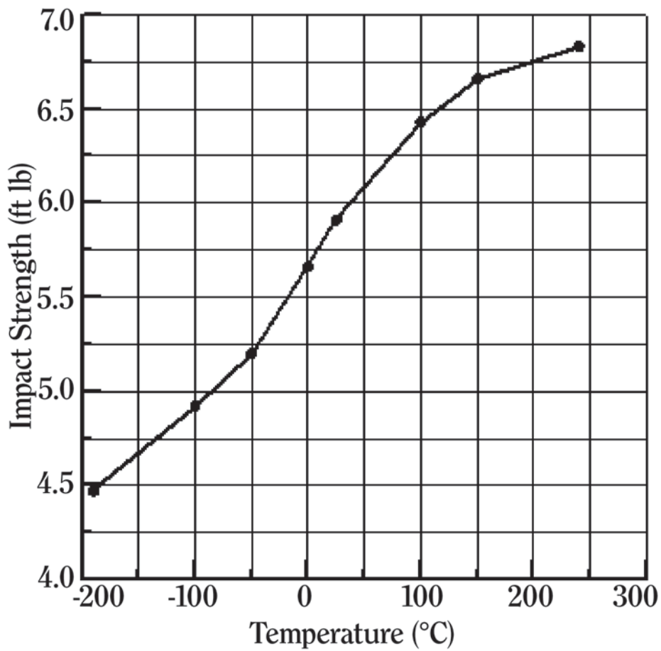
A380 Impact Strength at Temperature
